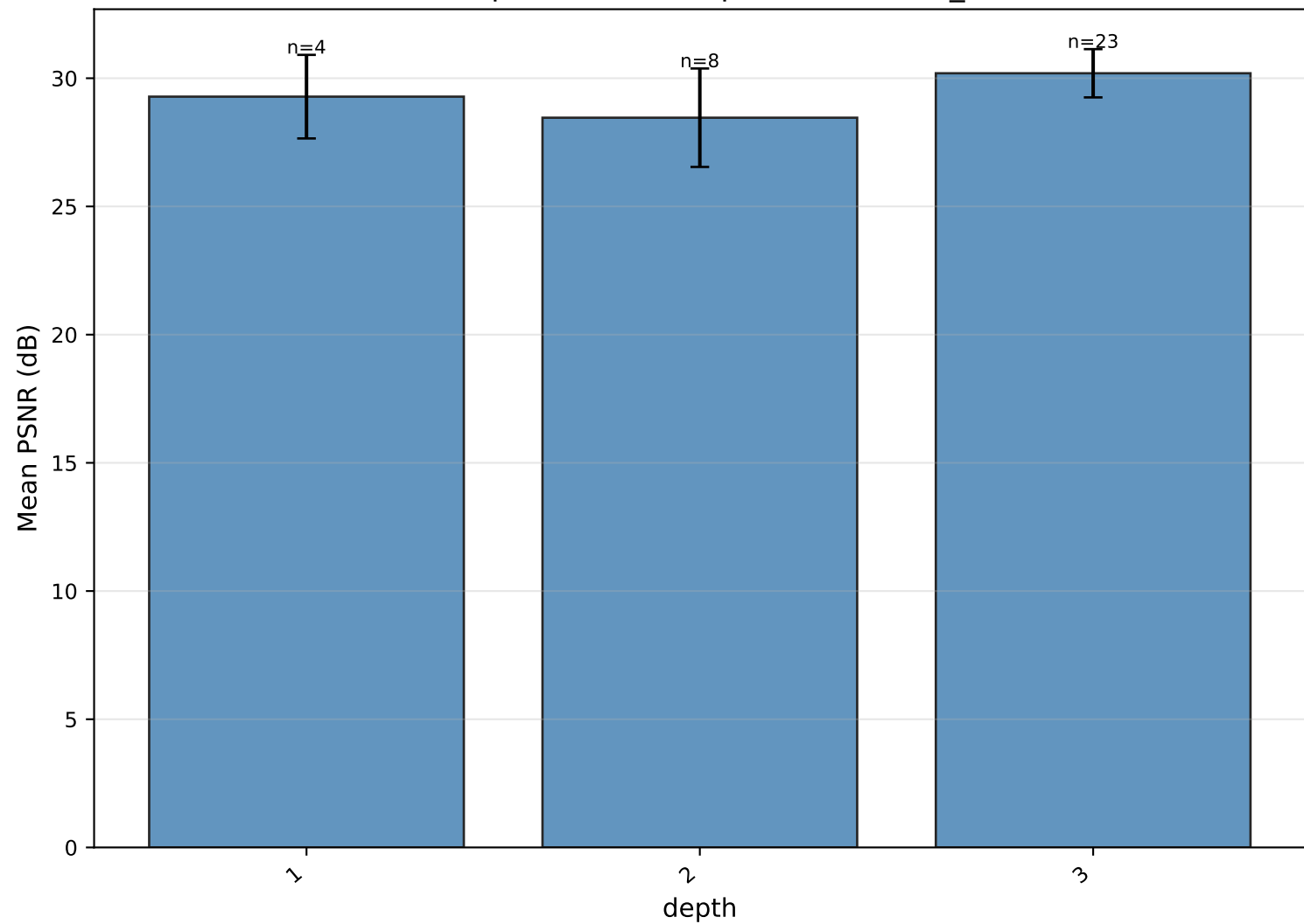
Mean PSNR per value of depth — DHTCUN_baseline
